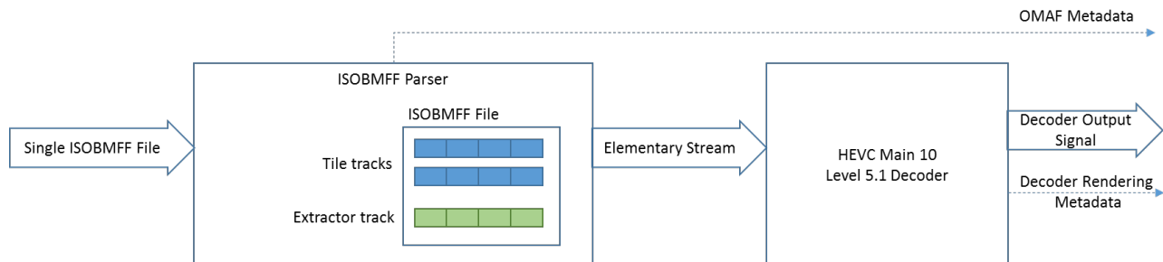
Figure 21: DASH Media Engine for HEVC-based viewport-dependent OMAF video profile
