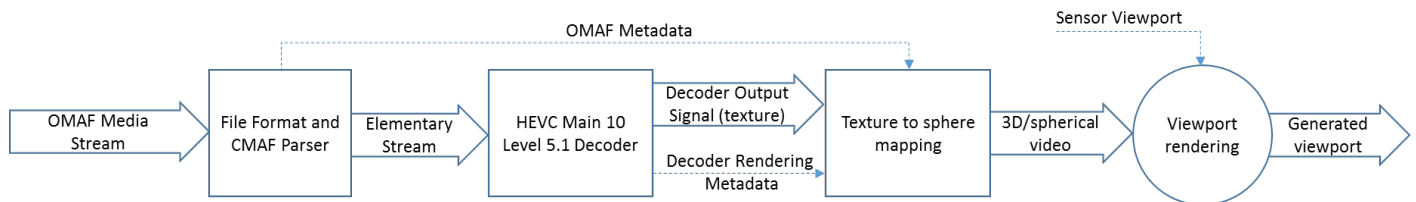
Figure 17: Logical Receiver Model
