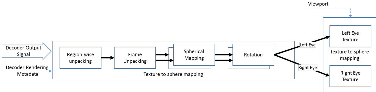
Figure 22: Inverse Projection/Renderer
